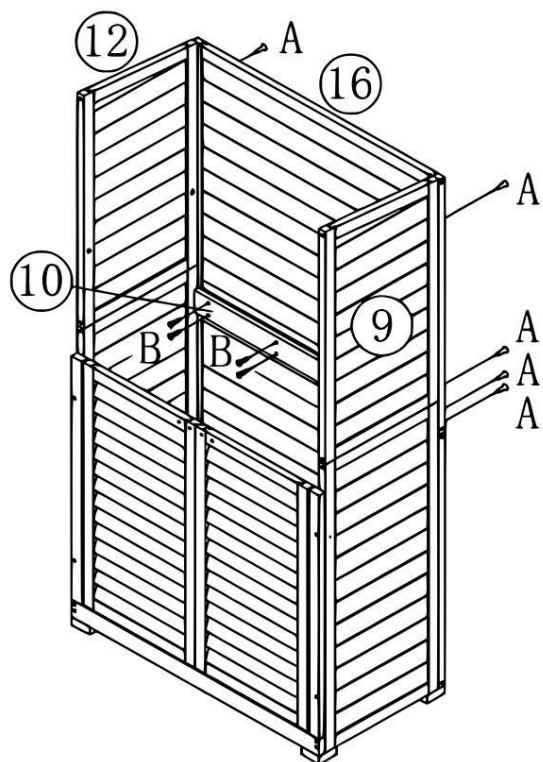
Krok 3 | A 3,5x40 mm (8) – B 3,5x30 mm (8)
