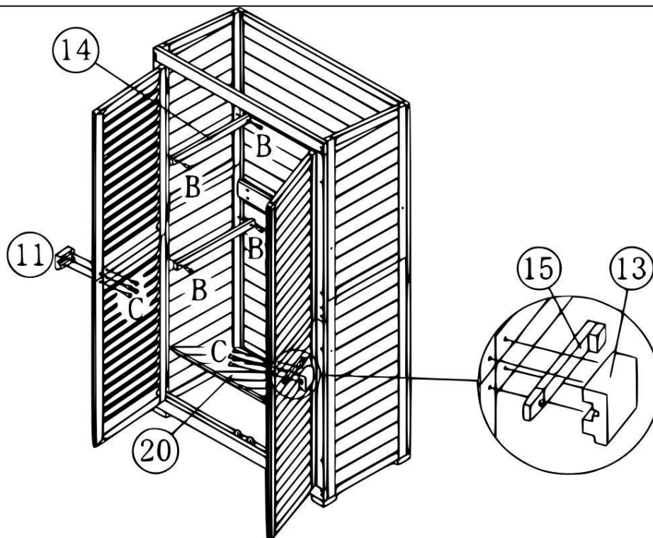
Krok 5 | B 3,5×30 mm (8) – C 3,5×35 mm (8)
